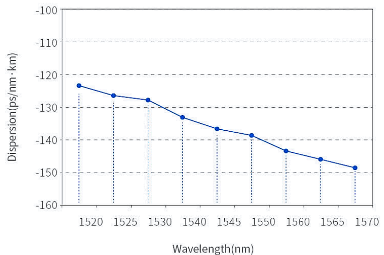
G.652 DCF Dispersion Curve
